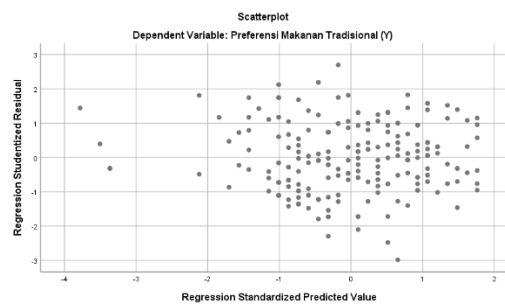
Figure 2. Dependent Variable
